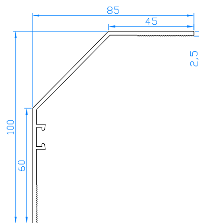
Abdeckwinkel 85x100 Code: 109.373
