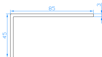
Abdeckwinkel 85x45 Code: 109.134
