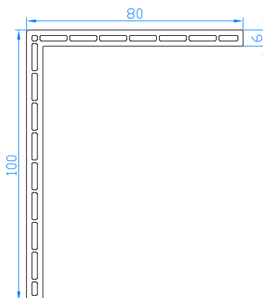
Abdeckwinkel 80x100 Code: 111.003
