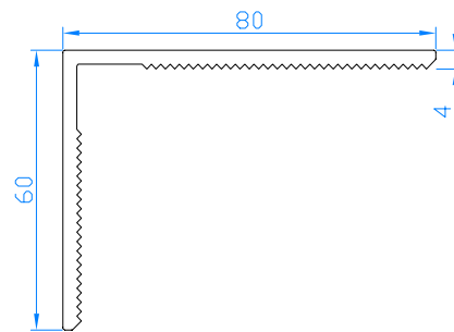
Abdeckwinkel 80x60 Code: 111.016
