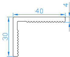
Abdeckwinkel 40x30 Code: 111.007
