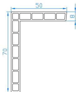
Abdeckwinkel 50x70 Code: 111.031
