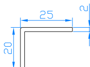
Abdeckwinkel 25x20 Code: 109.049
