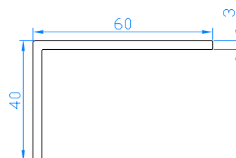
Abdeckwinkel 60x40 Code: 109.001
