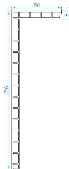
Abdeckwinkel 50x156 Code: 111.032
