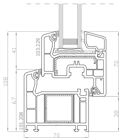
DPP-70 Lumia Line
