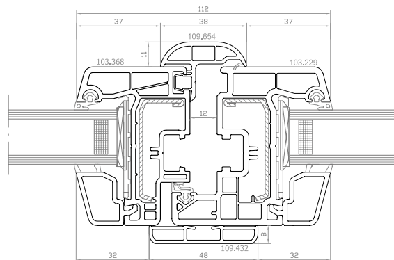
DPP-70 Lumia Line
