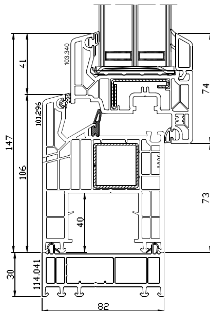
DPQ-82 H Anta 74mm
