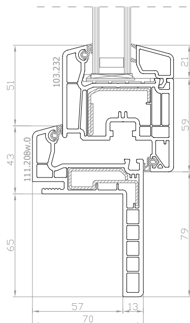
DPP-70 R65 telaio: 111.208w.0 anta: 103.232
