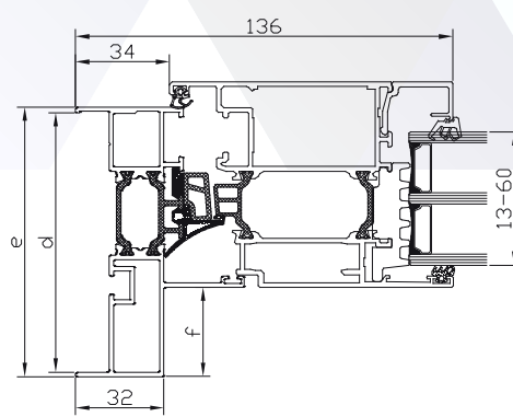
DA-65EF.M FW.../DA-65EF SW.03 MONOBLOC: 100, 120, 140, 160
