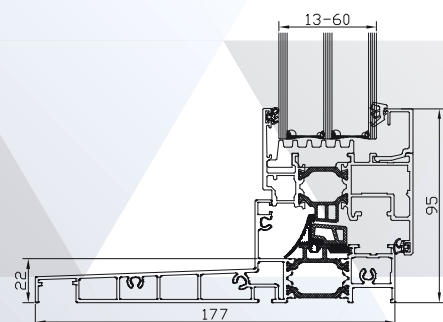
DA-65EF.M FW.10/DA- 65EF.SW.01 MONOBLOC: 100, 120, 140, 160
