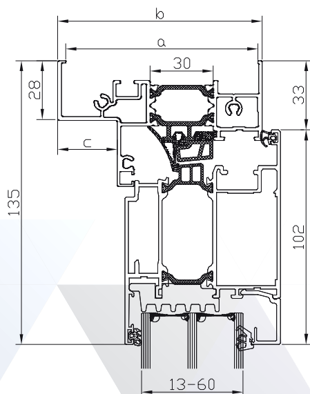
DA-65EF.M FW.../DA-65EF SW.03 MONOBLOC: 100, 120, 140, 160
