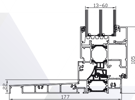
DA-65EF.M FW.10/DA-65EF. SW.02 MONOBLOC: 100, 120, 140, 160
