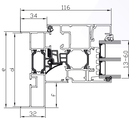
DA-65EF.M FW.../DA-65EF SW.02 MONOBLOC: 100, 120, 140, 160
