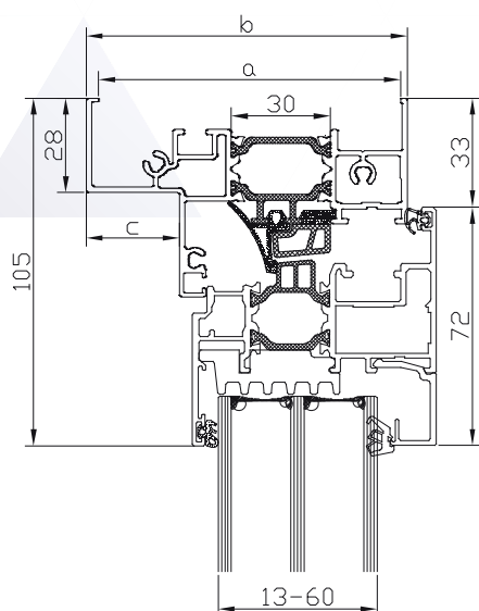
DA-65EF.M FW.../DA-65EF SW.01 MONOBLOC: 100, 120, 140, 160
