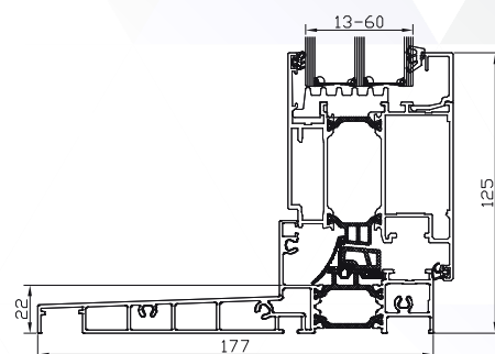
DA-65EF.M FW.10/DA-65EF. SW.03 MONOBLOC: 100, 120, 140, 160
