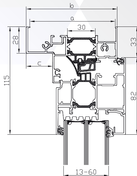
DA-65EF.M FW.../DA-65EF SW.02 MONOBLOC: 100, 120, 140, 160
