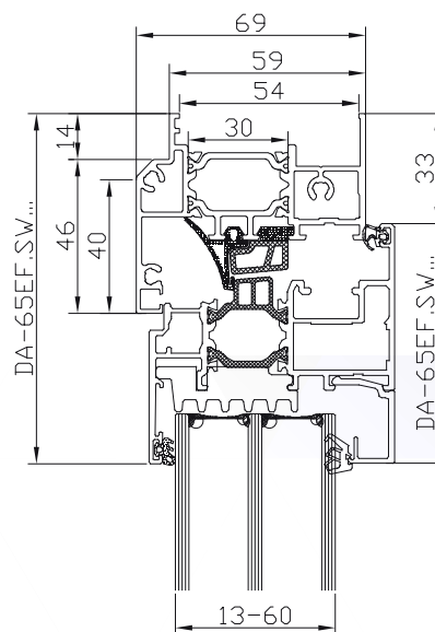
DA-65EF.M FW.05/DA-65EF SW... MONOBLOC: 100, 120, 140, 160
