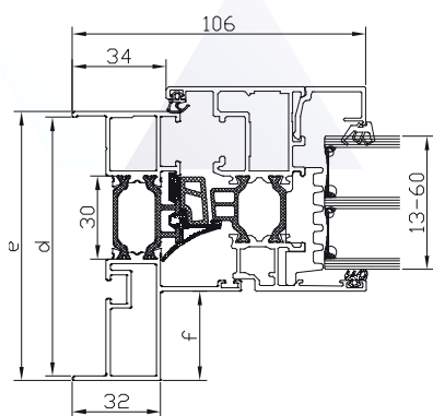
DA-65EF.M FW.../DA-65EF SW.01 MONOBLOC: 100, 120, 140, 160
