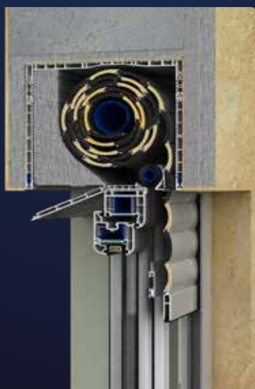
Top-mounted roller shutter in PVC box DK-RNB, DK-RNC
